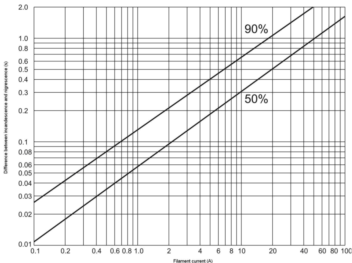
Figure 5 Correction Graph for Incandescence and Nigrescence Time
