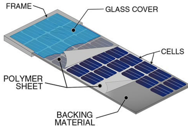
Figure 9 Figure showing the construction of a solar module from www.sunnetsolar.com
