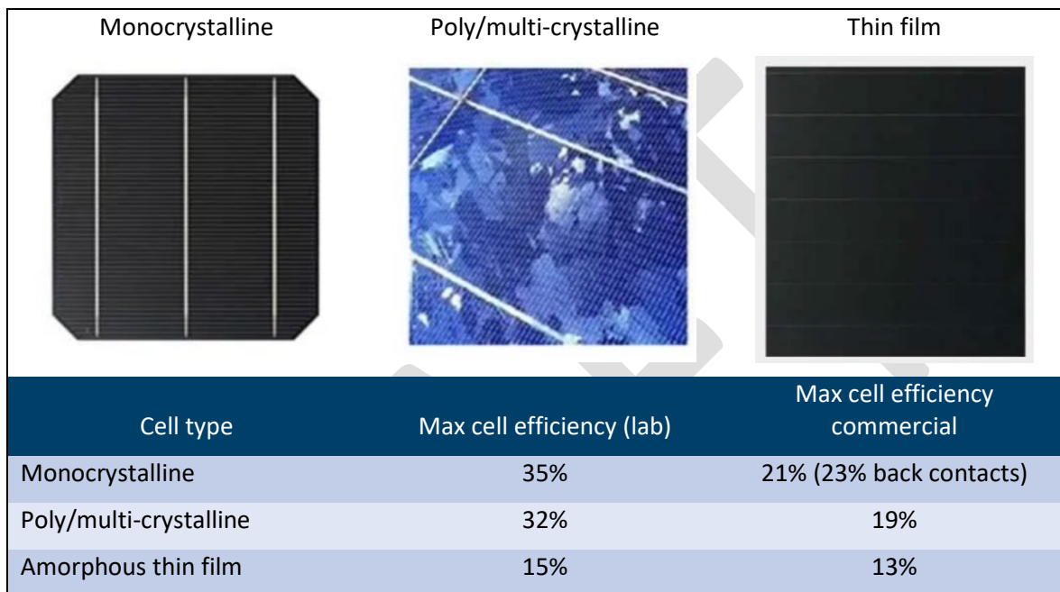
Figure 2 Types of solar cells
