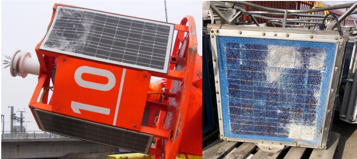
Figure 37 The effects of physical impact
