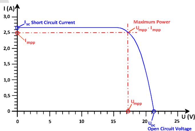
Figure 42 Current / voltage curve
