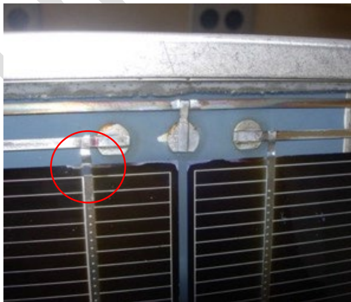
Figure 30 Ribbon fracture.
