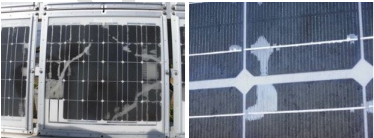
Figure 32 Examples of delamination.
