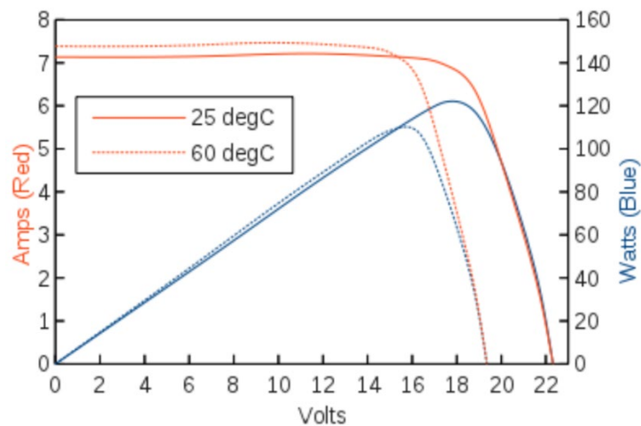
Figure 14 Impact of temperature on solar module performance
