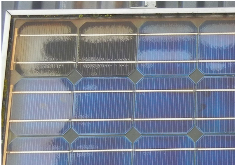
Figure 35 Encapsulant discolouration
