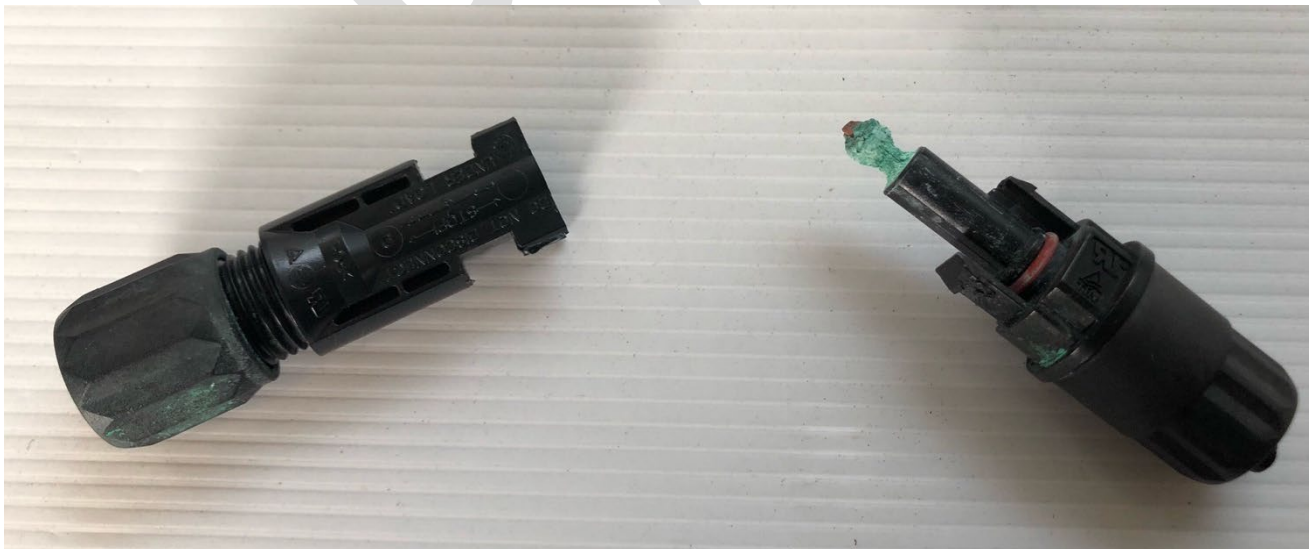
Figure 40 Connector failure
