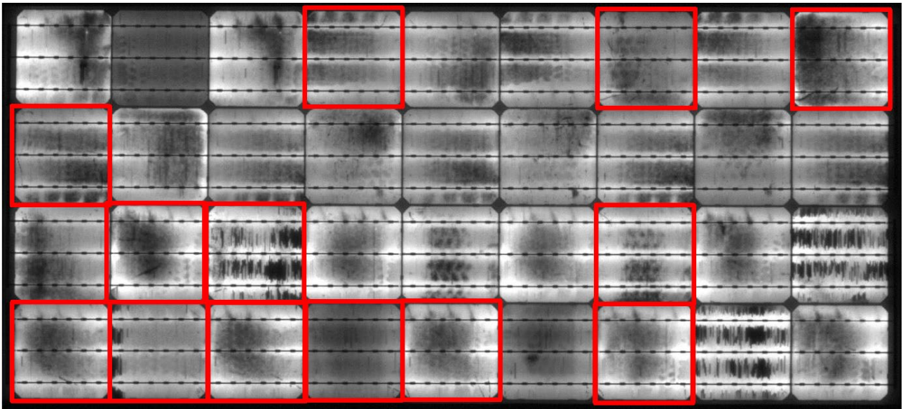
Figure 27 An example of a module with 13 cells which have micro cracking made visible using electro luminescence.
