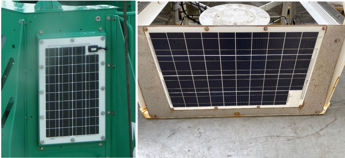
Figure 10 Showing the application of flexible solar module from Trinity House and Rijkswaterstaat
