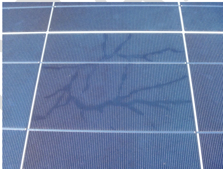
Figure 28 An example of Snails trails on a solar module (from the internet).
