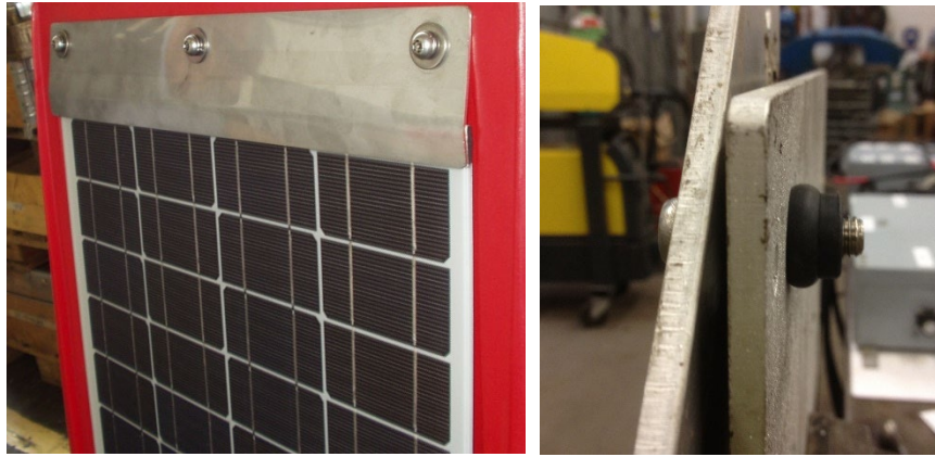
Figure 20 An example of direct fixing.
