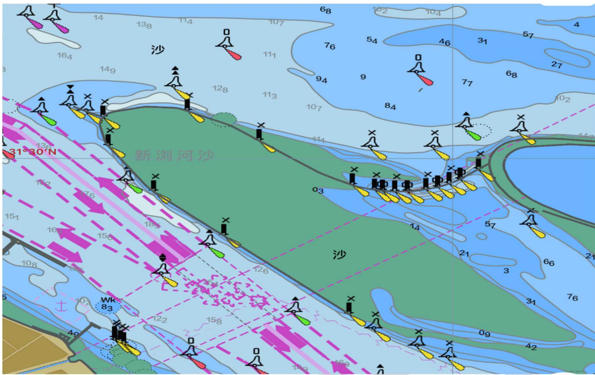
Figure 4 New Liuhe sand bar and Nanshatou Channel submerged breakwater (dikes), Yangtze River Estuary
