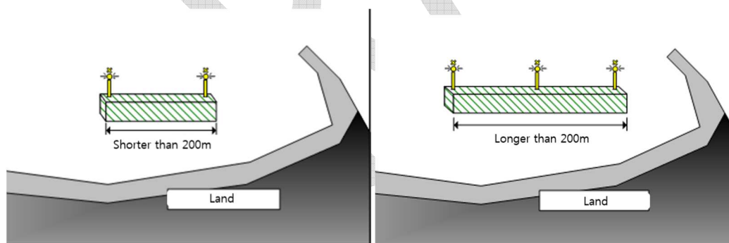
Figure 5 Example of marking breakwaters with fixed AtoN
