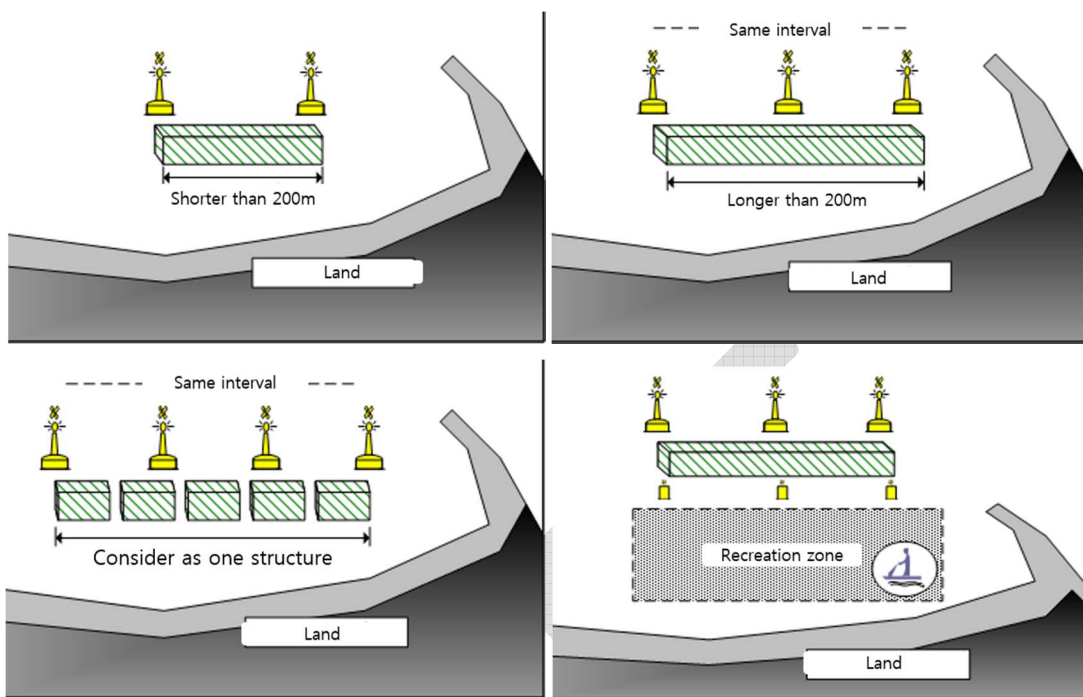
Figure 6 Examples of marking breakwaters with floating AtoN
