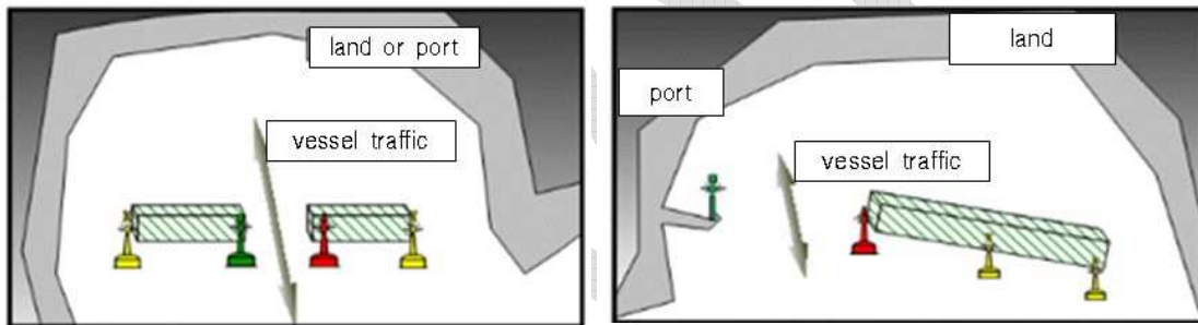
Figure 7 Example of marking passages between breakwaters or between breakwaters and the shore (IALA System B)
