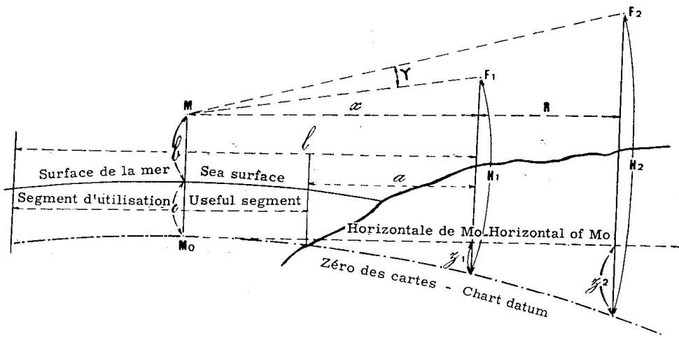
ELEVATION - VERTICAL SECTION
