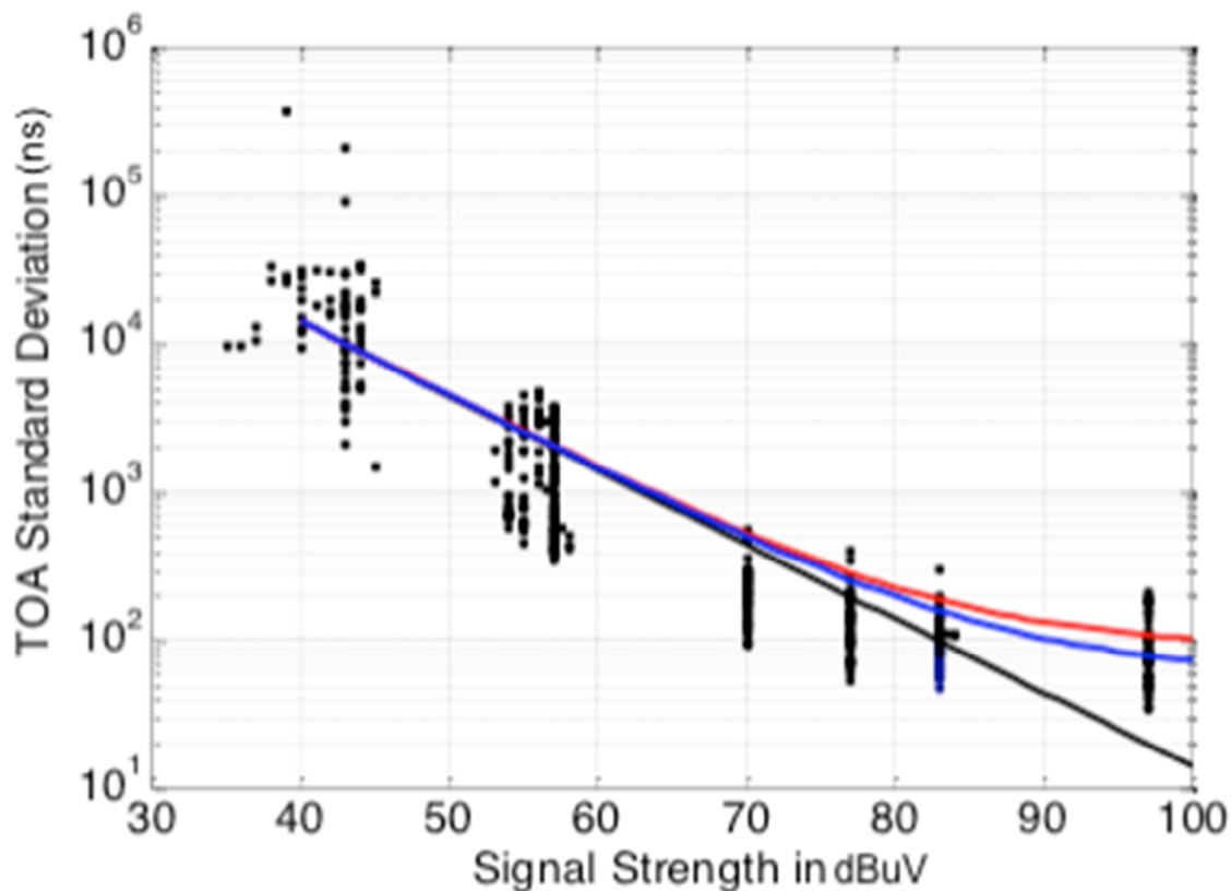
Figure 17: Typical performance of estimating the time of arrival from the eLoran signal as a function of the received signal strength in dB \mu V (reprinted from [7]).
