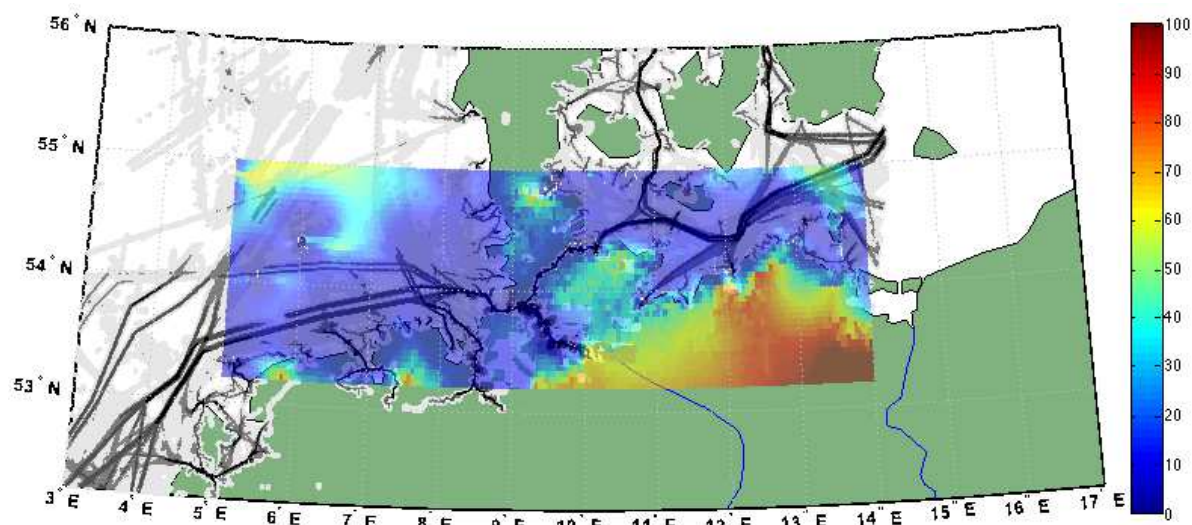
Figure 4: R-Mode performance overlaid on top of shipping density plot. Predicted R-Mode performance shaded using 0-100m accuracy scale. Shipping density shaded so that darker is higher density traffic.
