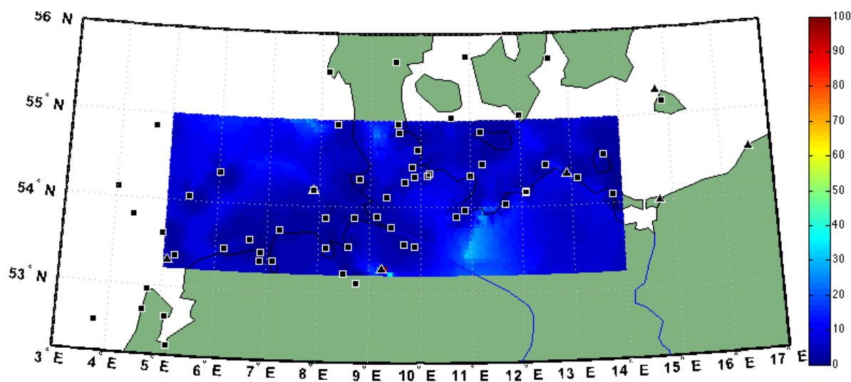
Figure 31: Lower bound to positioning accuracy of combined MF DGNSS and AIS R- Mode on region II– day. MF beacon locations are triangles, AIS stations are squares.
