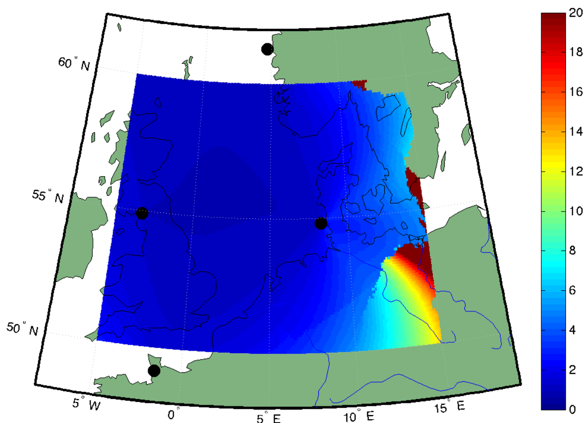
Figure 19: HDOP for the five eLoran stations in region I); Loran towers marked with black circles (Ejde is located to the NW just off the plot).
