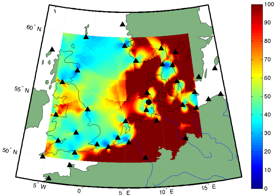
Figure 26: Lower bound to positioning accuracy of combined MF DGNSS and eLoran (Sytt only) on region I – night.
