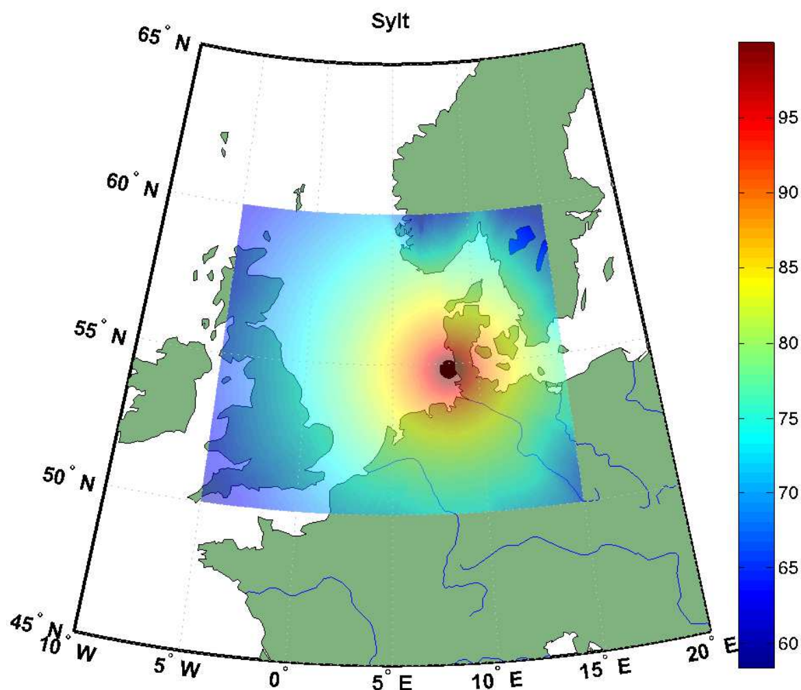
Figure 20: Predicted signal strength for a typical eLoran site, Sylt (in dBµV); Sylt is indicated by the black circle.
