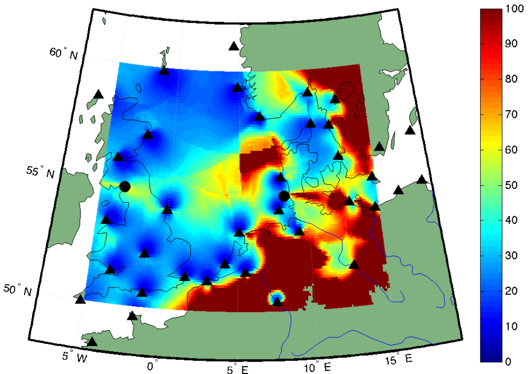
Figure 27: Lower bound to positioning accuracy of combined MF DGNSS and eLoran (Sytt and Anthorn) on region I - night.
